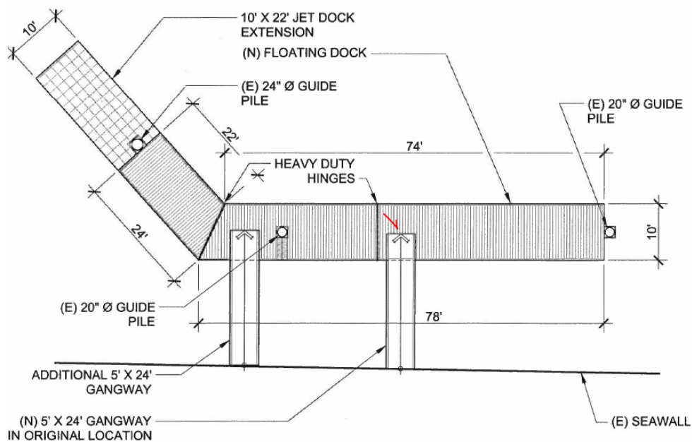
Figure 1: Swift Slip Dock & Pier Builder's Design
